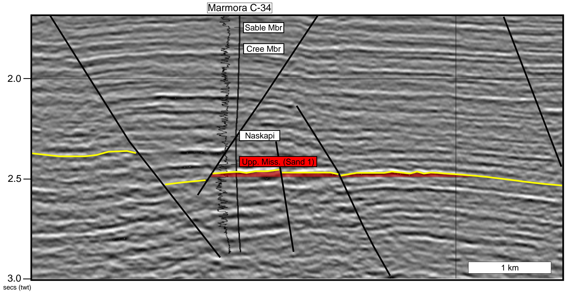
Inset box from figure 12, seismic profile near Marmora C-34 (well is projected 150 meters). The Sand 1 gas zone is shaded in red. The gamma ray log is shown to the left of the borehole.
